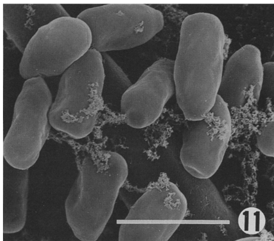
Figs. 9–11. Scanning electron micrographs of conidiogenous cells and conidia of L. pini-densiflorae .
